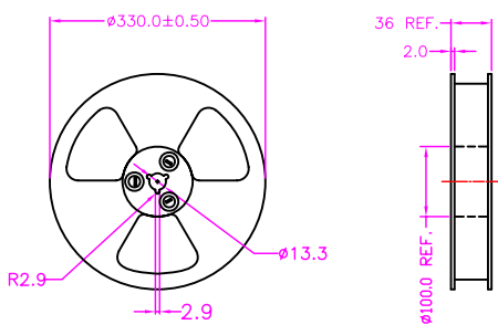
REEL FOR CARRIER TAPE
